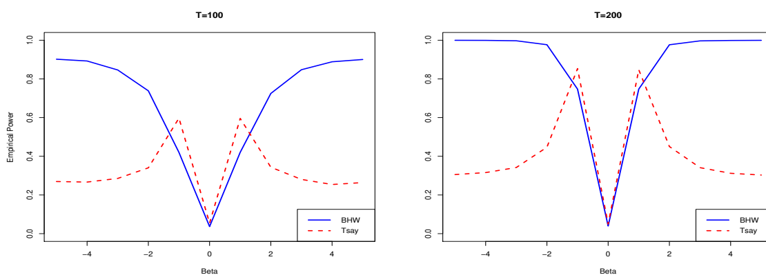
Figure 3: Empirical Power of Tsay's and BHW's Tests for different values of \beta in Model A.
