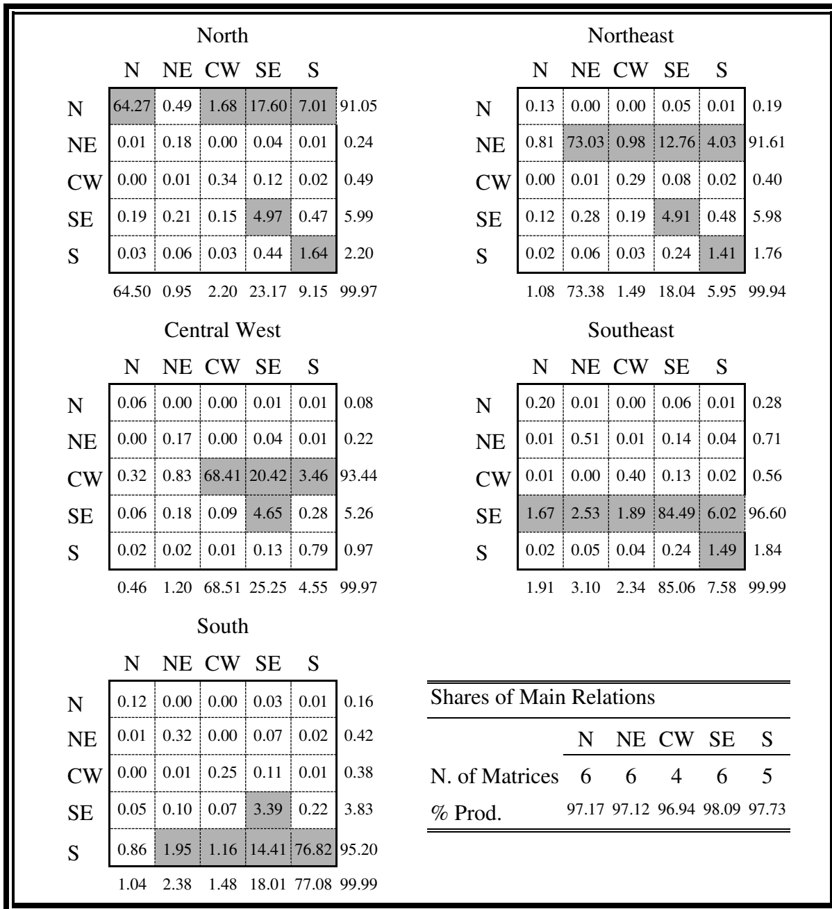
Figure 5. Contribution (%) of Each Block Matrix to the Total Share of (x_{l-f}) in x to the regions North, Northeast, Central West, Southeast, and South.
