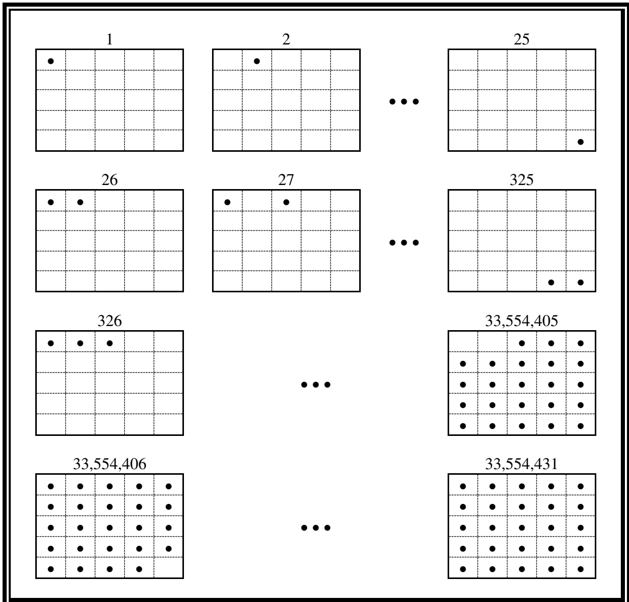
Figure 2. Schematic Representation of the Possible Forms of the A_l Matrix – 5 Regions Case.
