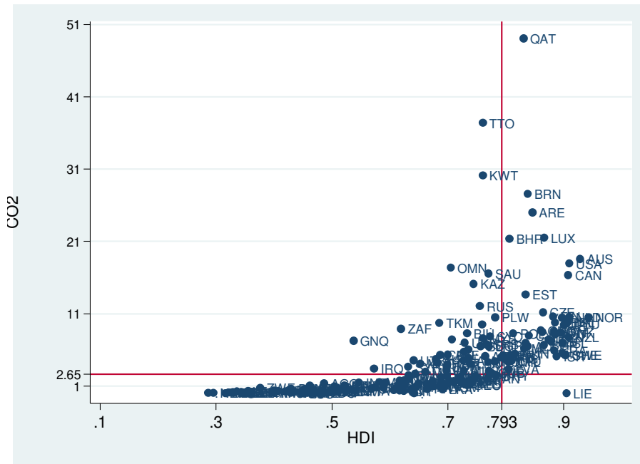
Figure A.2.3. Human Development Index and CO 2 emissions per capita (2008)
