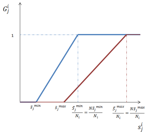
Figure A.1.2. Graphical representation of the loss function G_j^i with a minimum and a maximum planetary boundary
