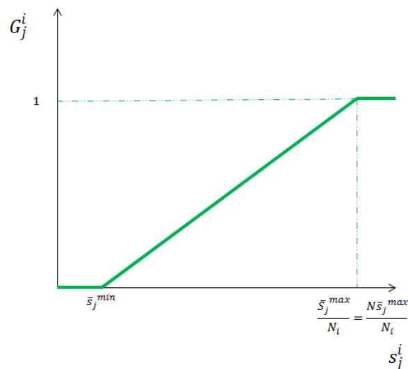
Figure A.1.3. Graphical representation of the loss function G_j^i with the minimum per capita fair share and the maximum global planetary boundary
