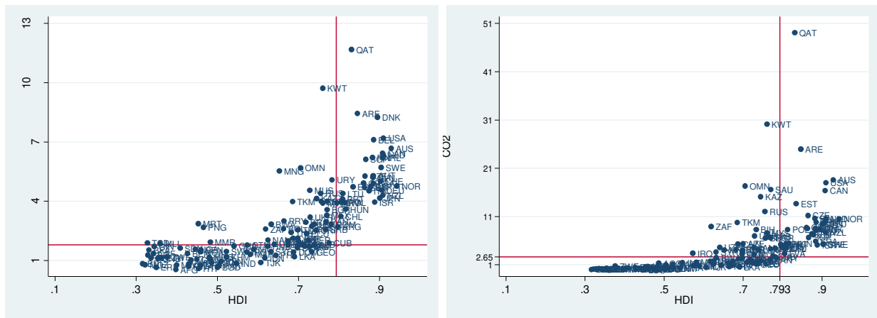
Figure A.2.7. Human Development Index, CO 2 emissions per capita and Ecological Footprint (2008) (Common sample, 140 countries)
