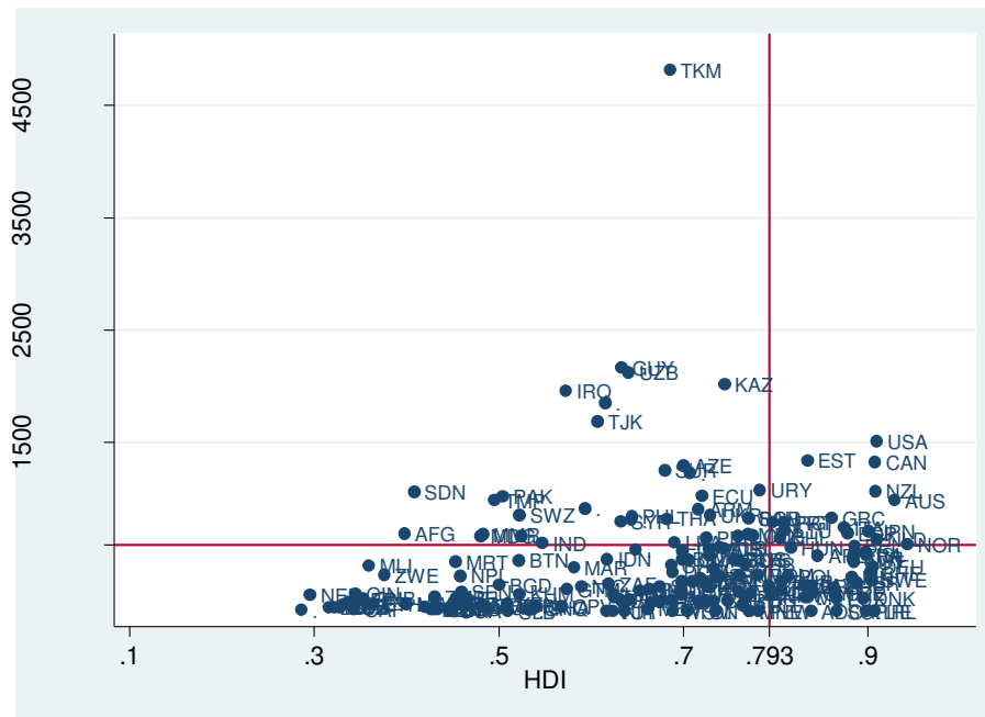
Figure A.2.4. Human Development Index and fresh water withdrawals per capita (2009)
