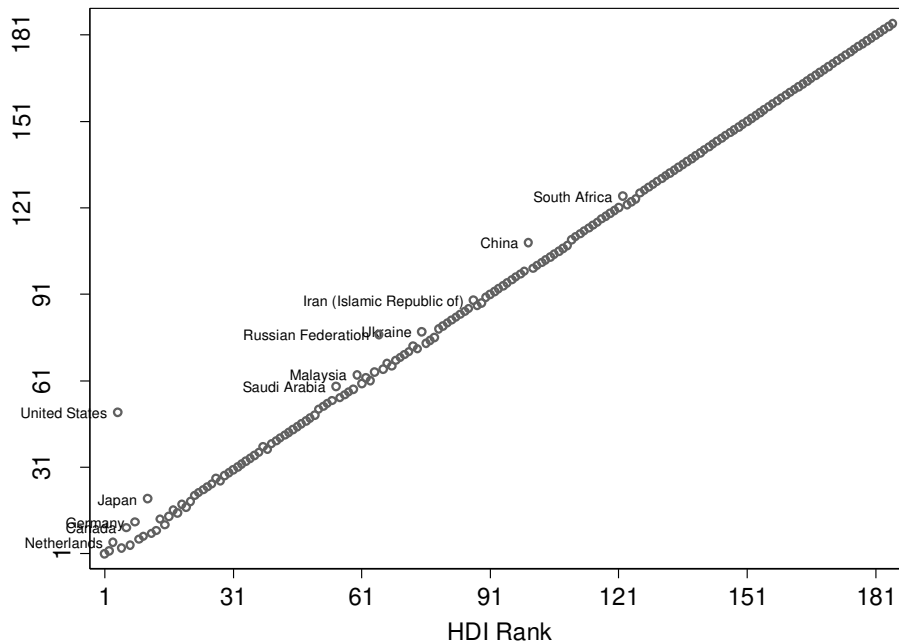
Figure 3. Rank comparison between HDI and SHDI (at the upper boundary).
