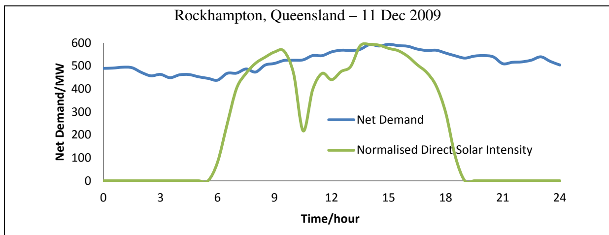
Figure 5 Comparing normalised direct solar intensity to the highest peak demand day in 2007-2011 at 5 nodes in the NEM
