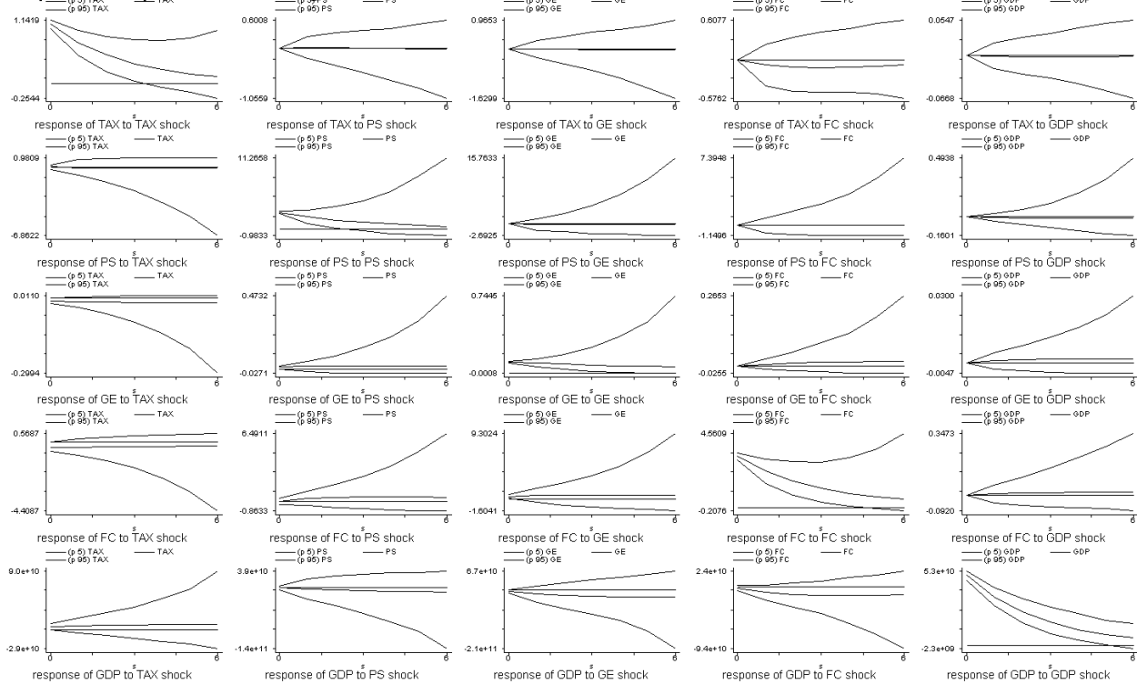
Errors are 5% on each side generated by Monte-Carlo with 1000 reps
