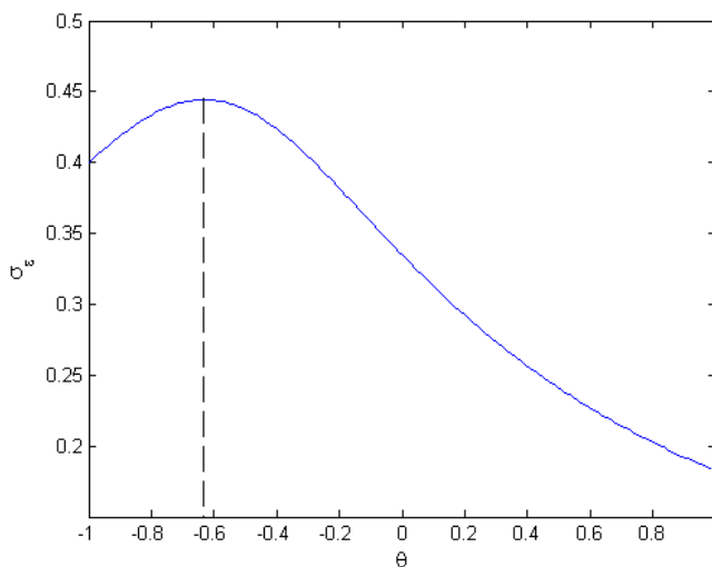
Figure 2. The maximum of \sigma_\varepsilon for different \theta in (-1,1)
