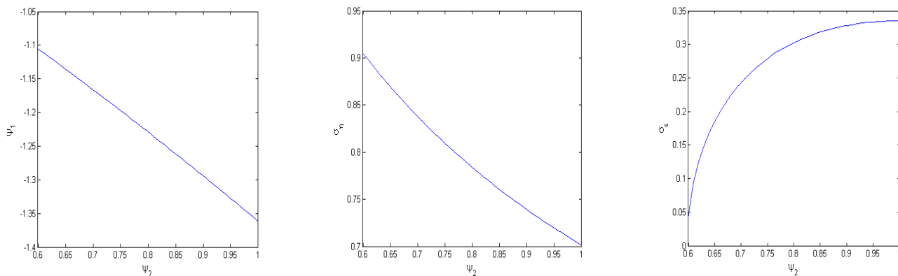
Figure 1 —The relationship between \{\psi_1, \sigma_\eta, \sigma_\varepsilon\} and \psi_2 when \theta = 0
