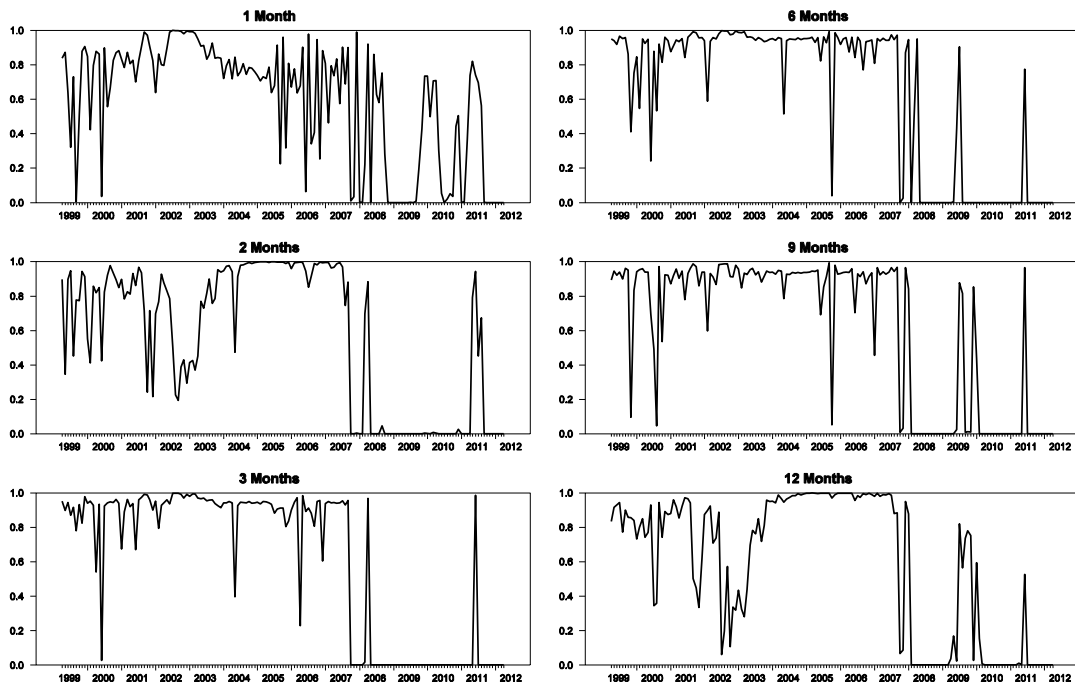
Figure 3b. Smoothed transition probabilities for Regime 2
