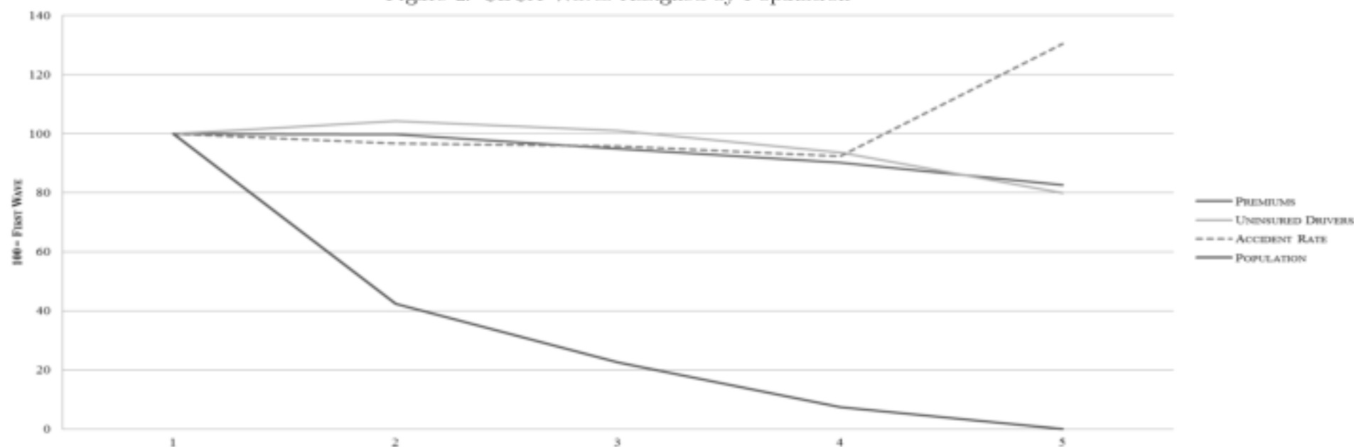
Figure 2: CLCA Waves Assigned by Population
