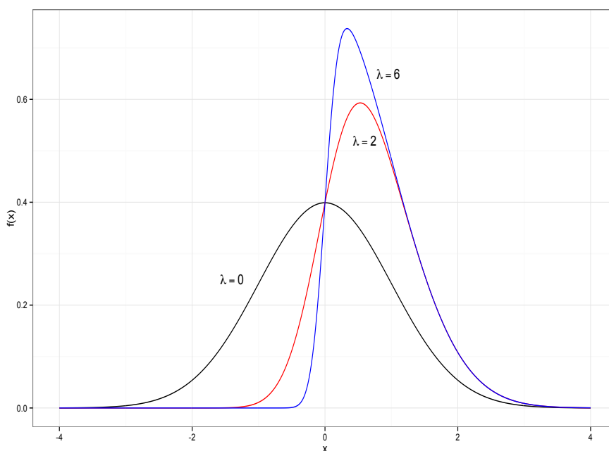
Figure 2: The Skew-Normal Distribution \lambda = 0, 2, 6
