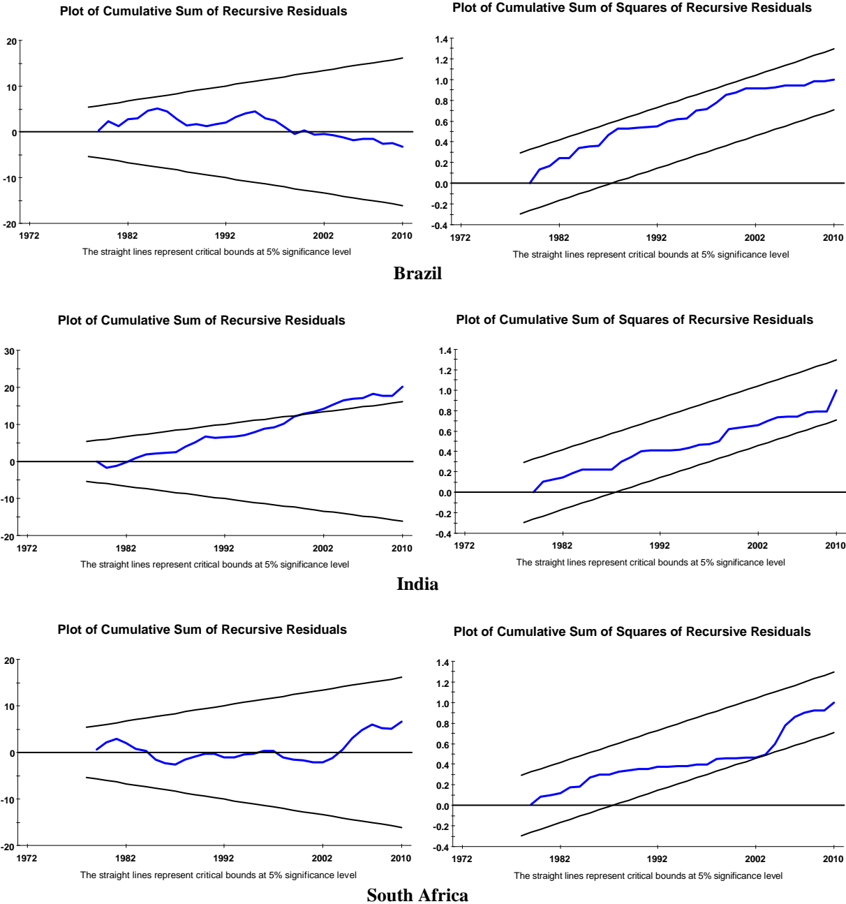
Figure 2. Plots of CUSUM and CUSUMQ tests
