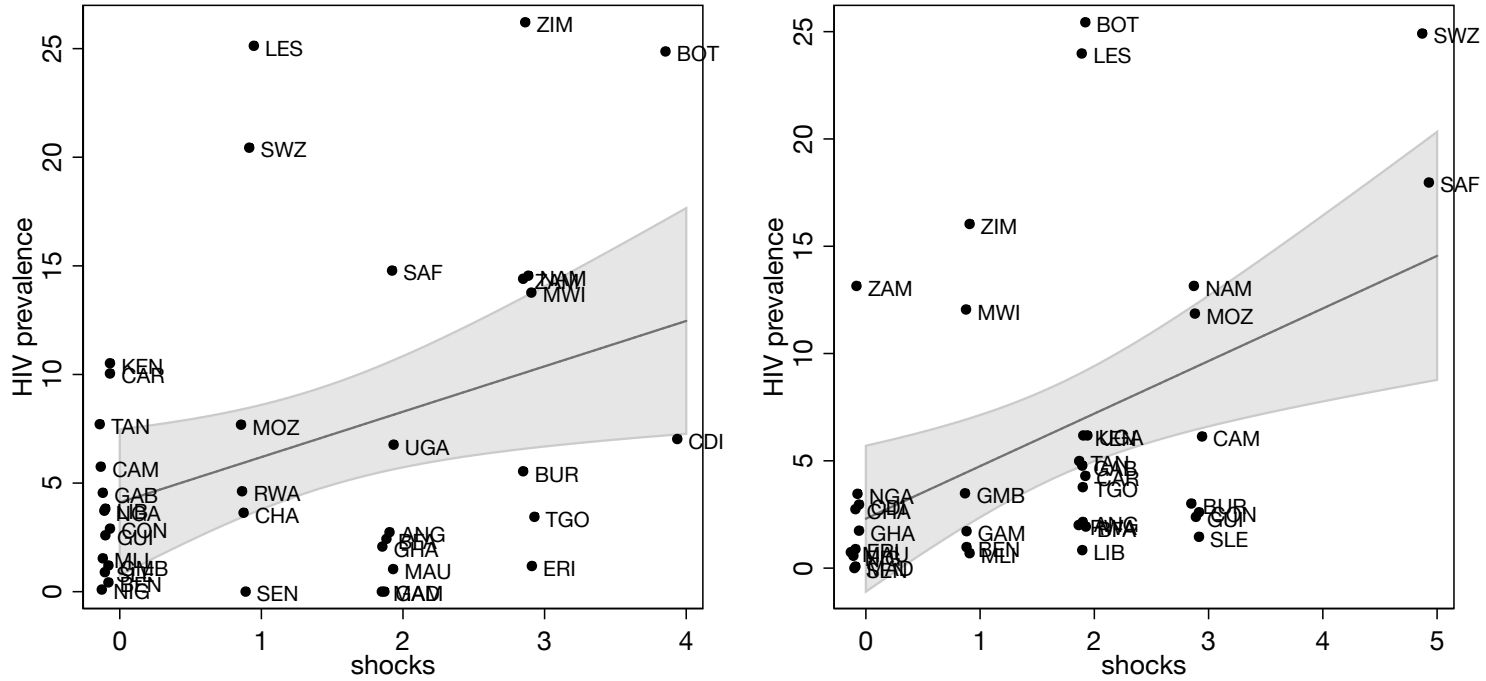
Figure 3: Country-level HIV prevalence & Shocks
