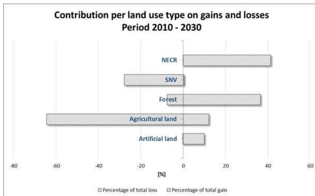
Figure 17. Gains and losses of aggregated land-use classes, at European level and under the A1B Scenario
