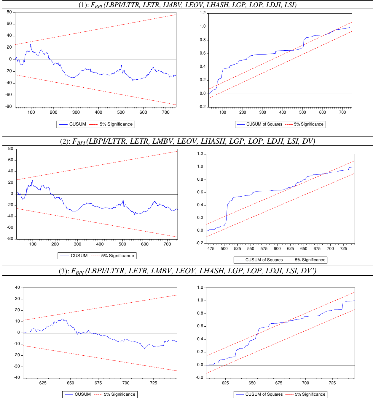
Figure A-1: Plots of cumulative sum of recursive and of squares of recursive residuals (Equations with additional variables)
