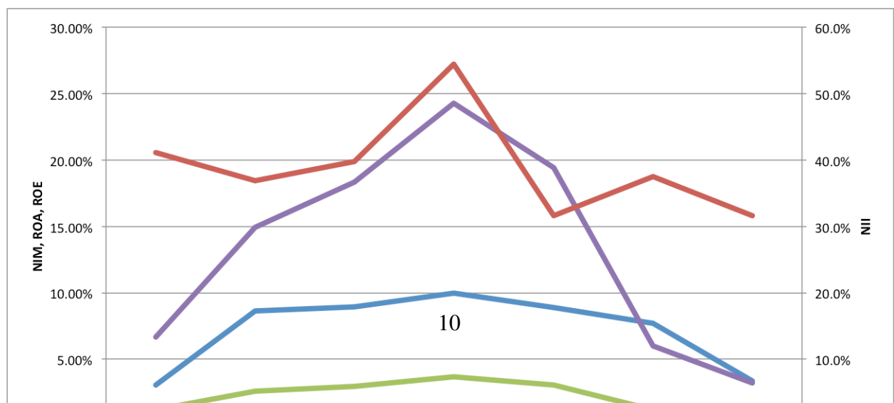
Figure 1 : Evolution of NIM, ROA, ROE and NII
