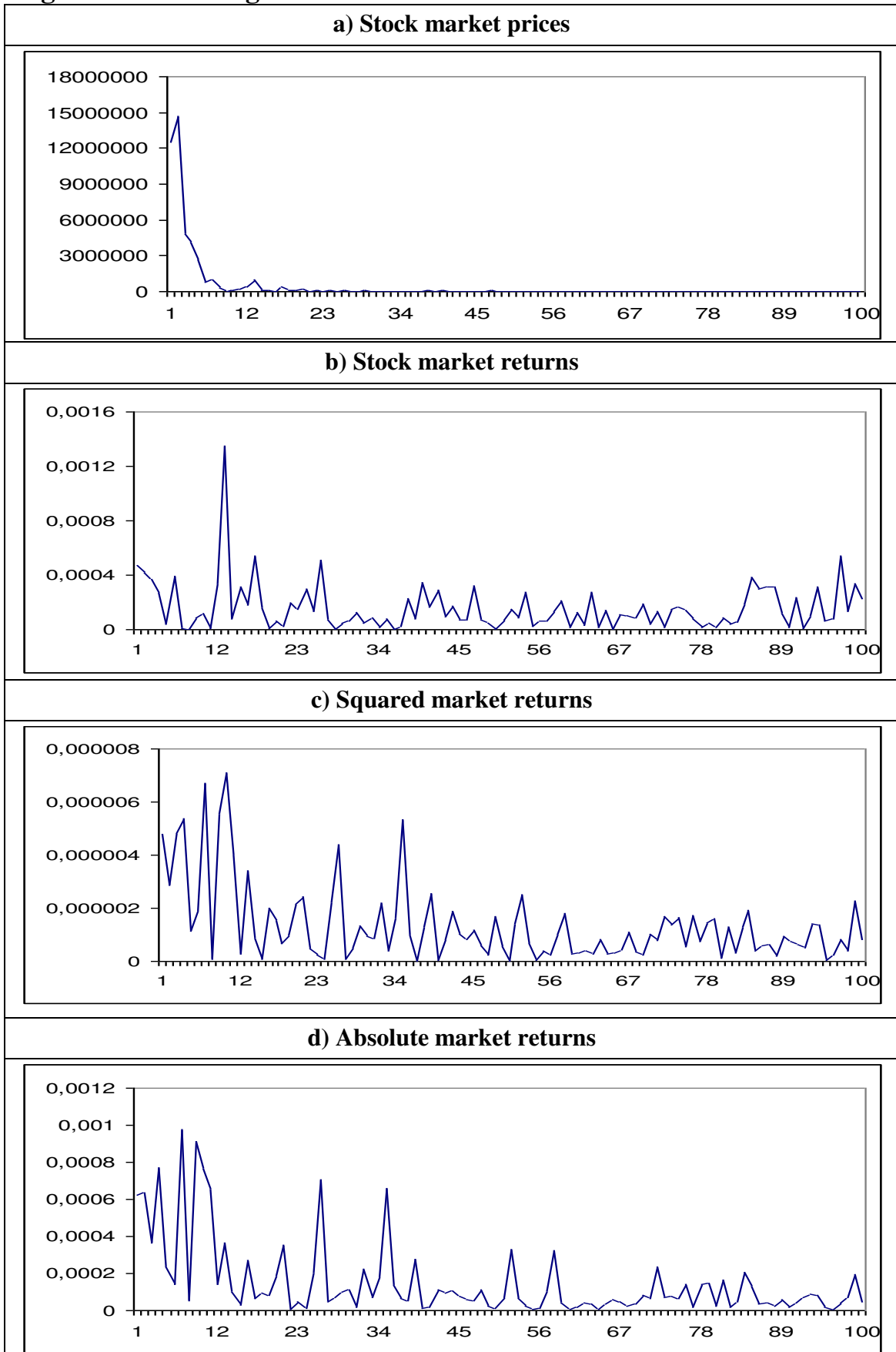
Figure 12: Periodograms
