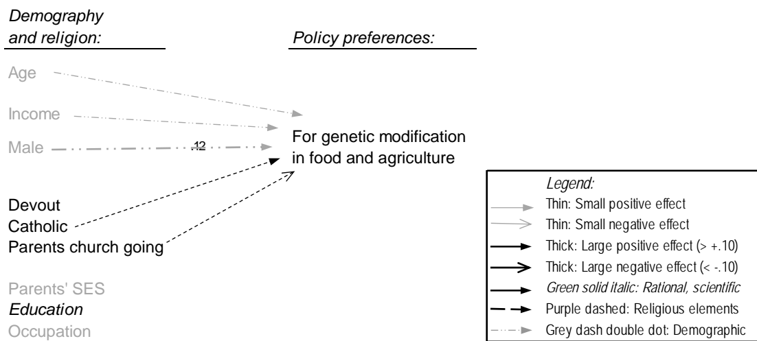
Fig. 2. Total effects of demographic and religious variables on policy preferences about genetic modification in food and agriculture. Only statistically significant effects (at p < .01 ) with standardized effects greater than .05 are shown
