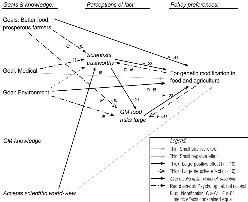
Fig. 5. Effects of perceptions of fact (concerning how trustworthy scientists are about GM and how risky GM food is) on policy preferences for genetically modified food and agriculture. Model with reciprocal causation (paths C and F). For simplicity, effects of demographic and religious variables, which are few and small, are not shown here (they are in Table 3)
