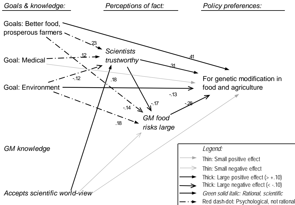
Fig. 4. Effects of perception of fact (concerning how trustworthy scientists are about GM and how risky GM food is) on policy preferences for genetically modified food and agriculture. Simple recursive model without reciprocal causation. For simplicity, effects of demographic and religious variables, which are few and small, are not shown
