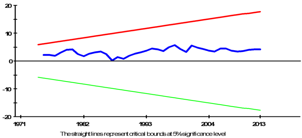
Plot of Cumulative Sum of Recursive Residuals
