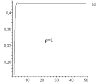
(b) Cyclical convergence to the stable steady state
