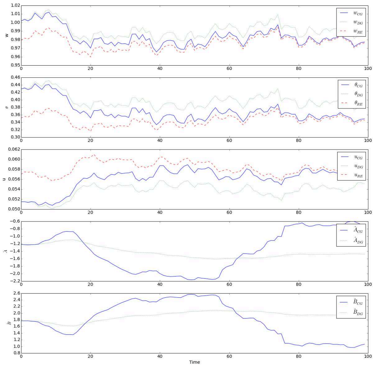
Figure 7: Learning (IV) - Comparison of decreasing and constant gain learning
