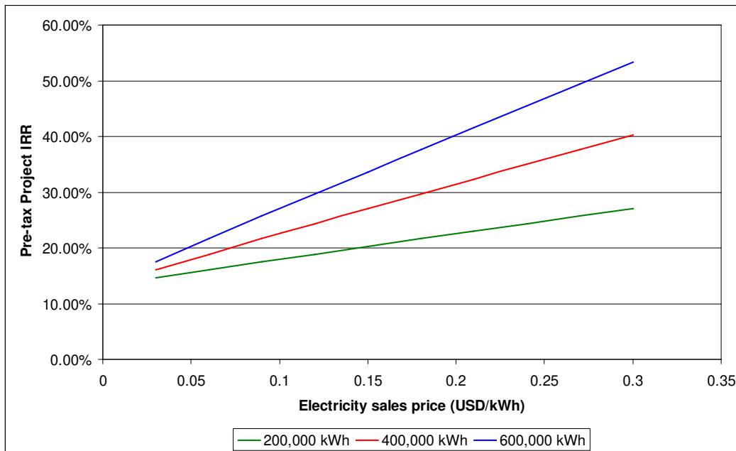
Figure 2 Feasibility study 200 kW methan-fired power generation plant
