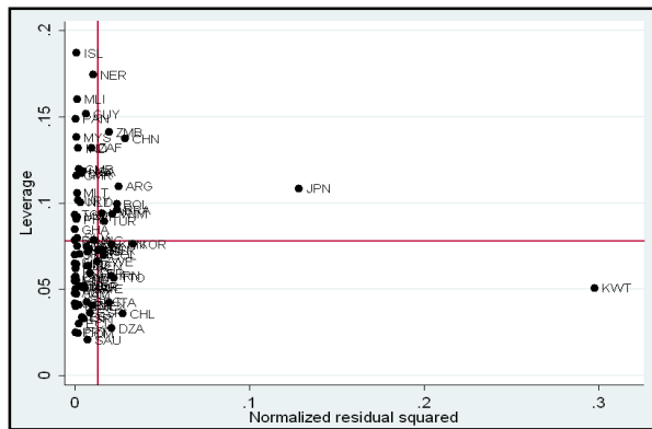
Figure 2. Residual versus leverage
