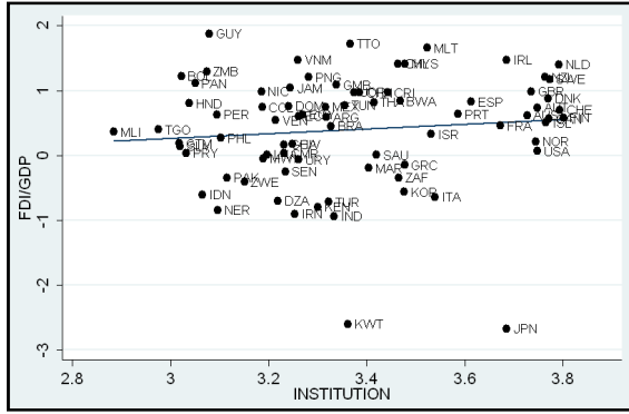
Figure 1. Scatter plot of FDI versus its Determinants
