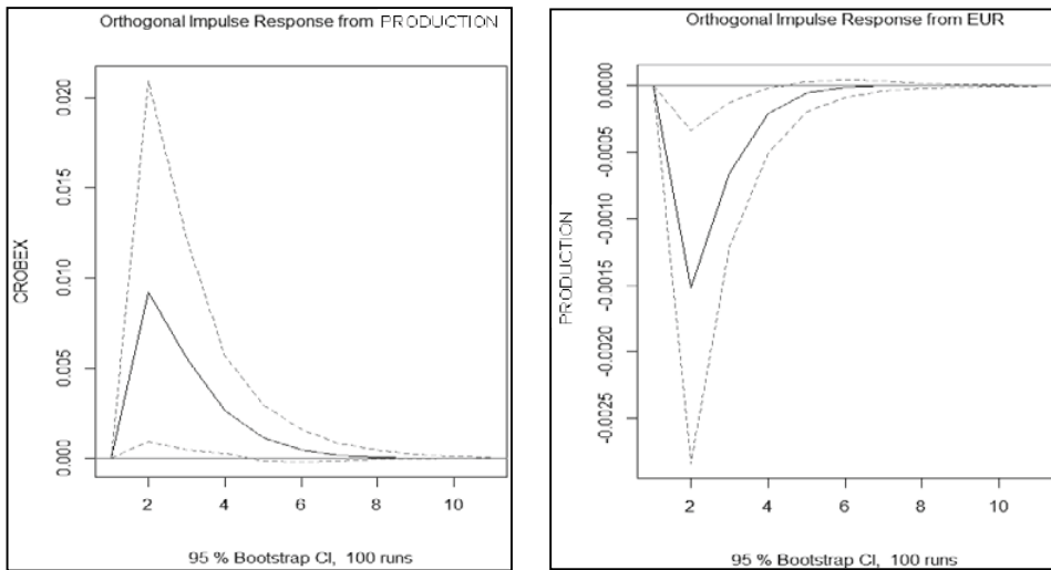
Picture 2: Function of impulse response for the CROBEX variable (left picture) and function of impulse response for the PRODUCTION variable (right picture)
