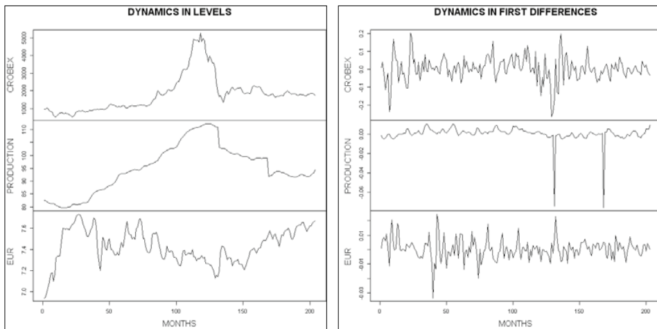
Picture 1.: Comparative overview of the time series variables CROBEX , PRODUCTION and EUR time series in levels (left), comparative overview of their first differences (right)
