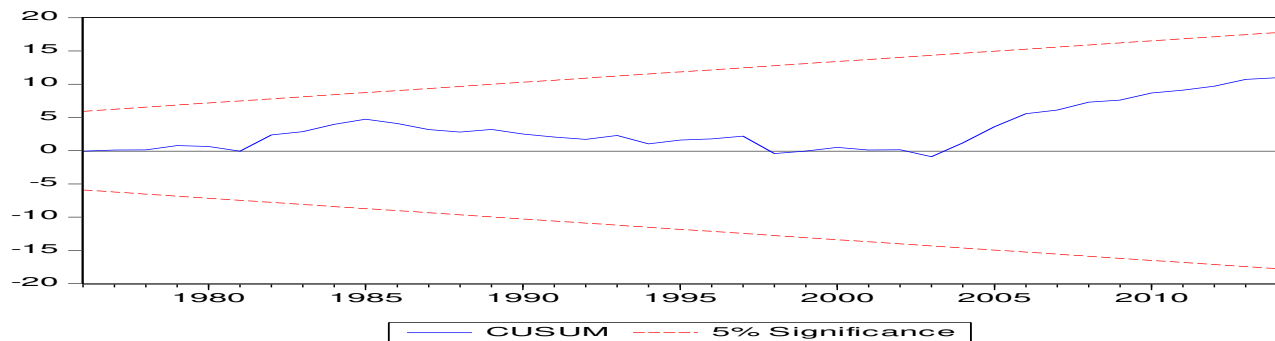
Figur-1: Plot of Cumulative Sum of Recursive Residuals
