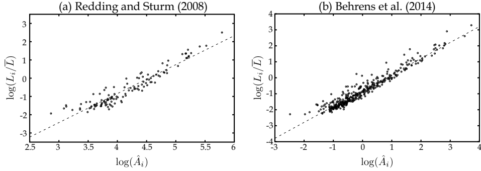
Figure 9: The relationship between city sizes and the estimated unobserved amenities
