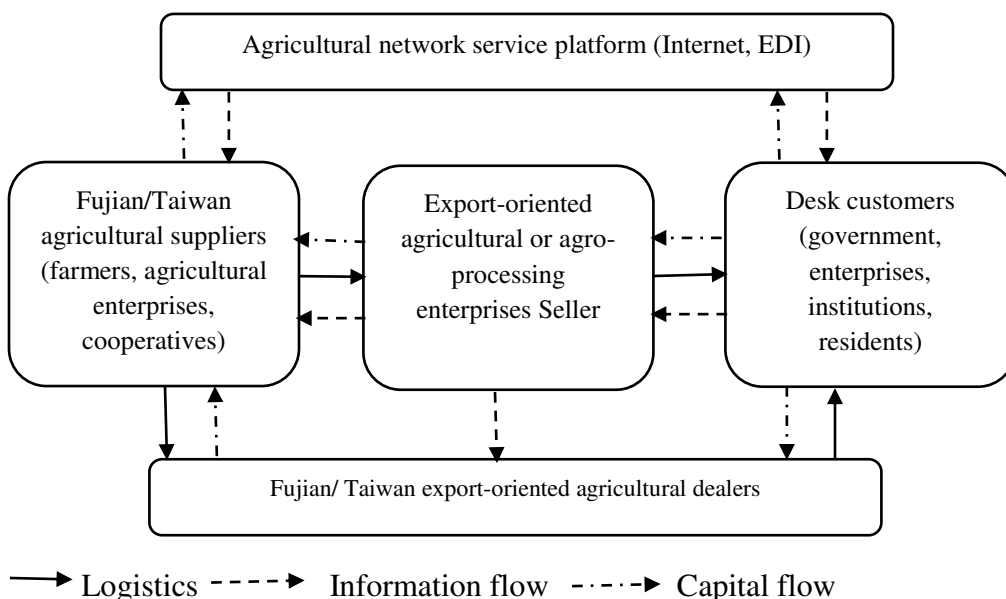
—→ Logistics - - - - -> Information flow - · - · - ·> Capital flow Figure 1. Network Analysis Based on Supply Chain Management of Agricultural Technology Innovation between Fujian and Taiwan
