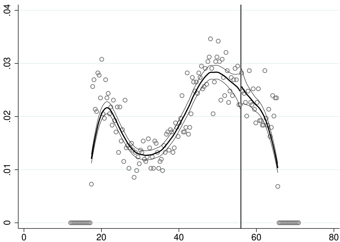
Figure 3: Density of the Forcing Variable: McCrary Test
