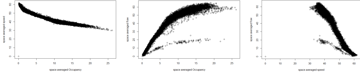
Figure 6: MFD for Geneva city. Left most picture represent the relation between speed and occupancy, middle picture represents flow and occupancy and the right most picture represents speed and flow relationship for the month of September 2014
