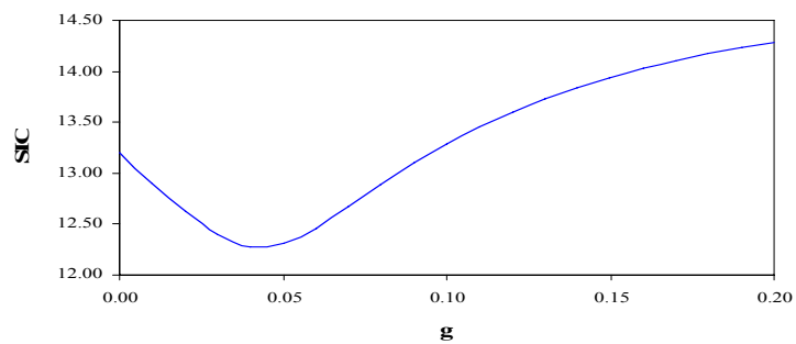
Fig. 4. Calculated SIC for the values of g
