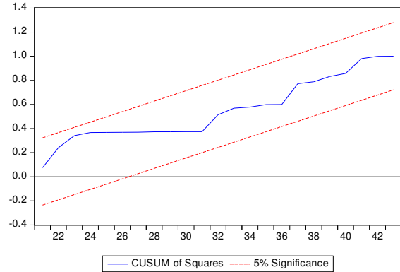
Figure 4.6: CUSUMSQ Test
