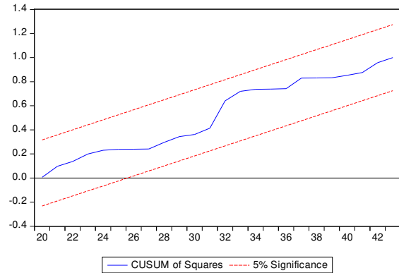
Figure 4.8: CUSUMSQ Test
