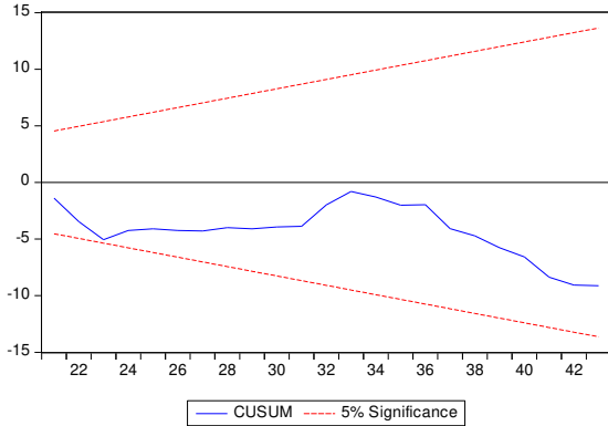
Figure 4.5: CUSUM Test
