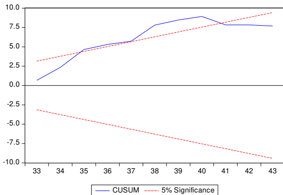
Figure 4.15: CUSUM Test
