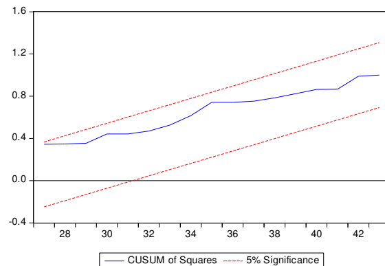
Figure 4.12: CUSUMSQ Test
