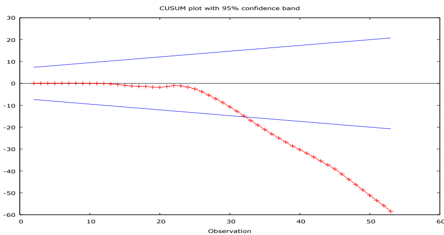
Figure 6. Plot of CUSUM
