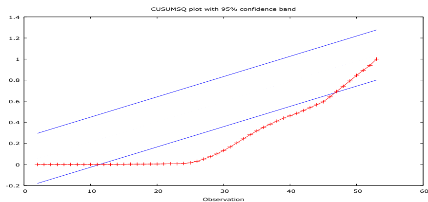
Figure 7. Plot of CUSUMSQ
