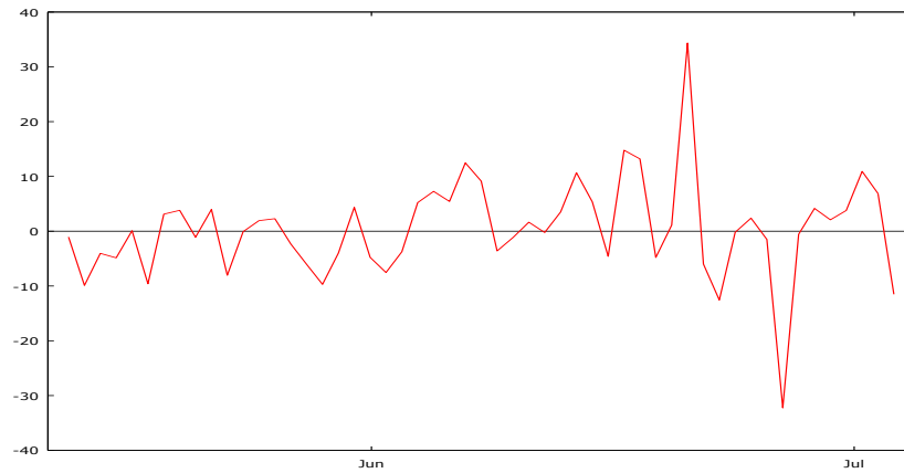
Figure 3. Time Series Plot of TO (1 st diff.)
