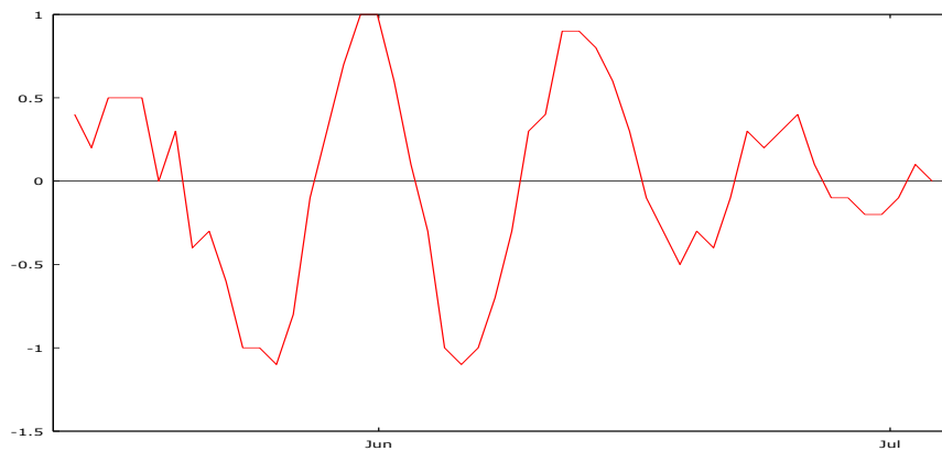
Figure 5. Time Series Plot of POV (2 st diff.)
