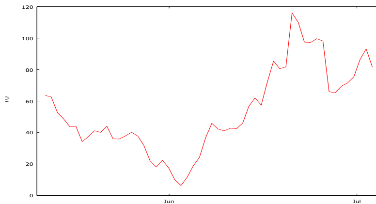
Figure 1. Time Series Plot of TO (levels)
