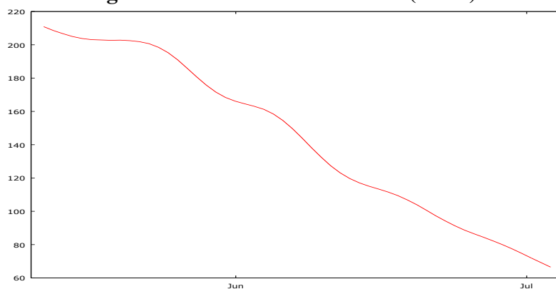
Figure 2. Time Series Plot of POV (levels)
