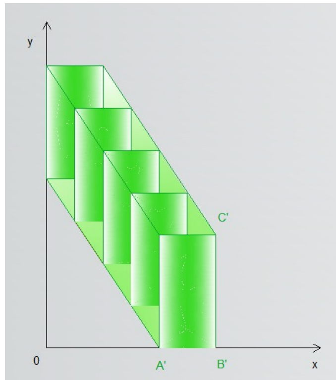
Figure 4: Payoff space of the game (f, <) .
