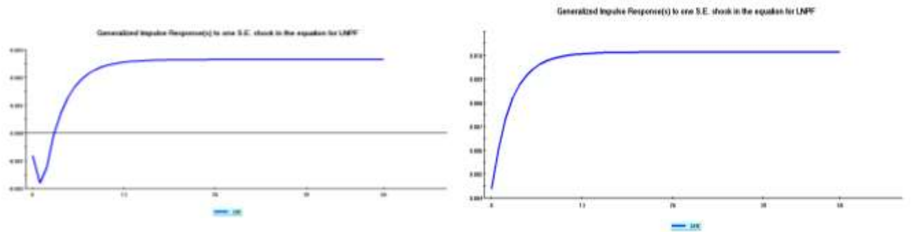
Figure 6: Generalize impulse response to one SE shock in the equation for LNPL
