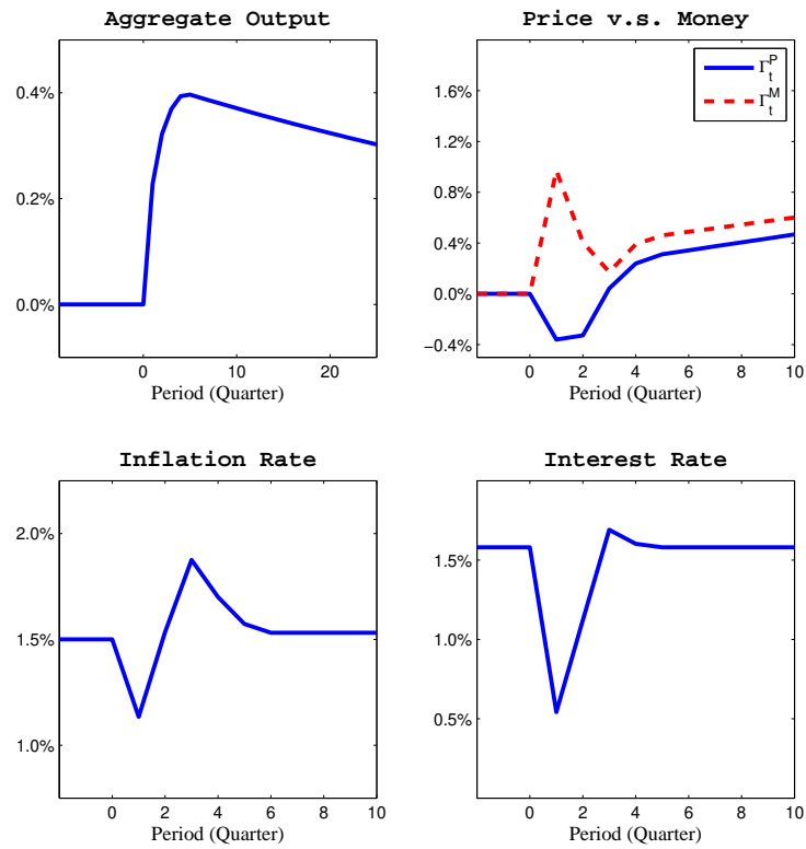
Figure 12: Transitional paths following a 1.667% money injection, N = 5 .
