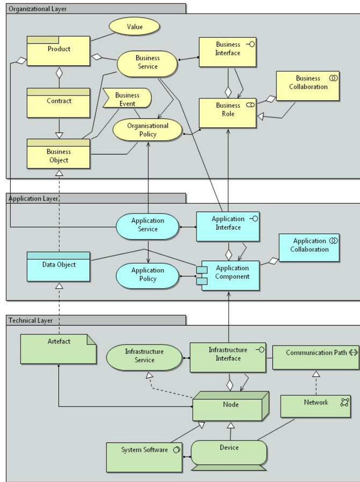
Figure 2. Smart monitoring platform metamodel
