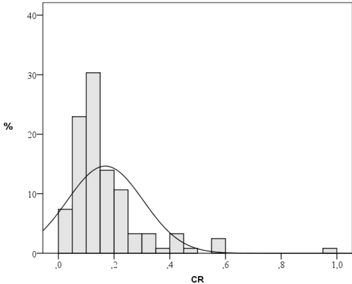
Figure 1. The distribution of the Consistency Ratio (CR) values of experts' ratings
