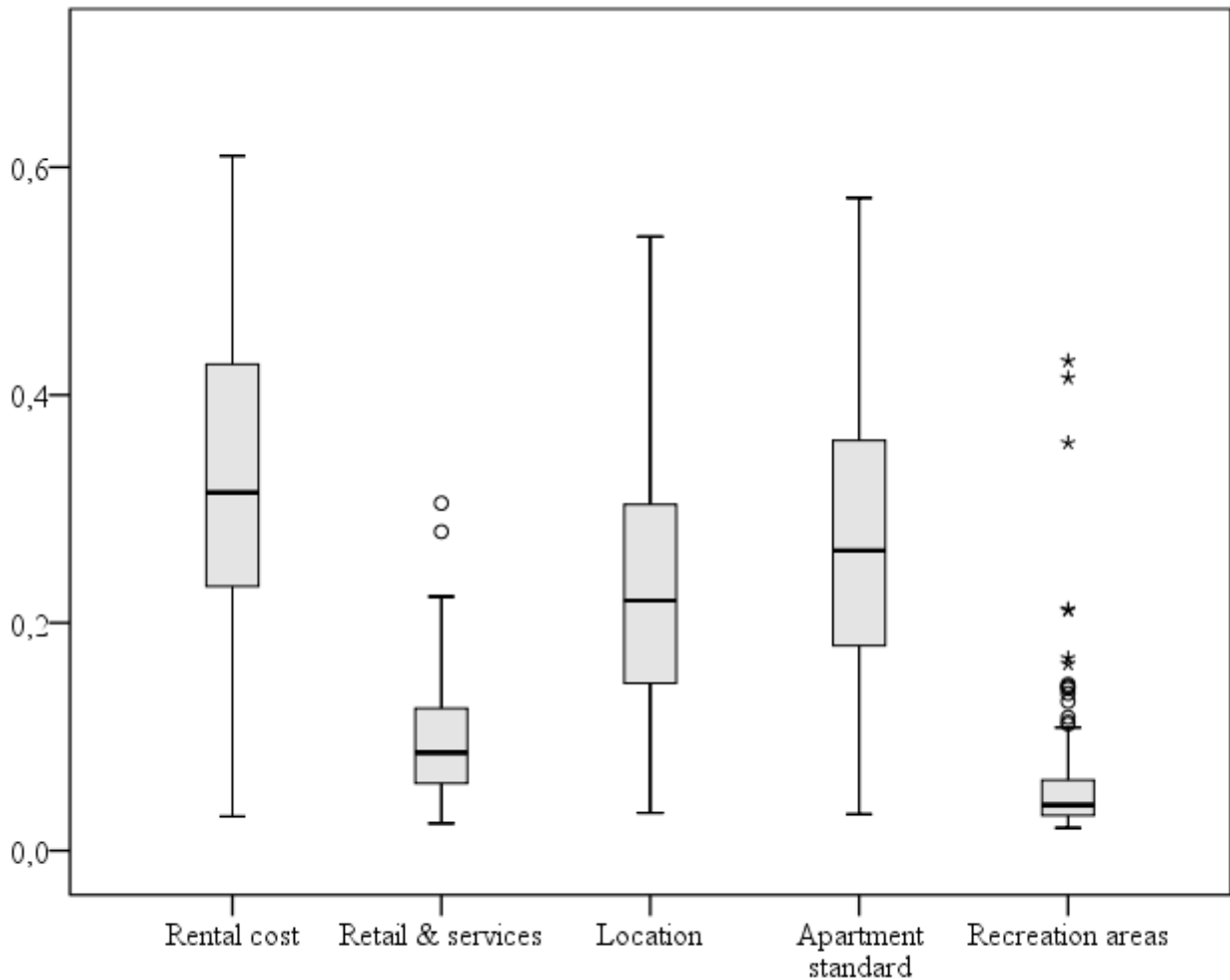
Figure 2. Distribution of experts' criterion weights
