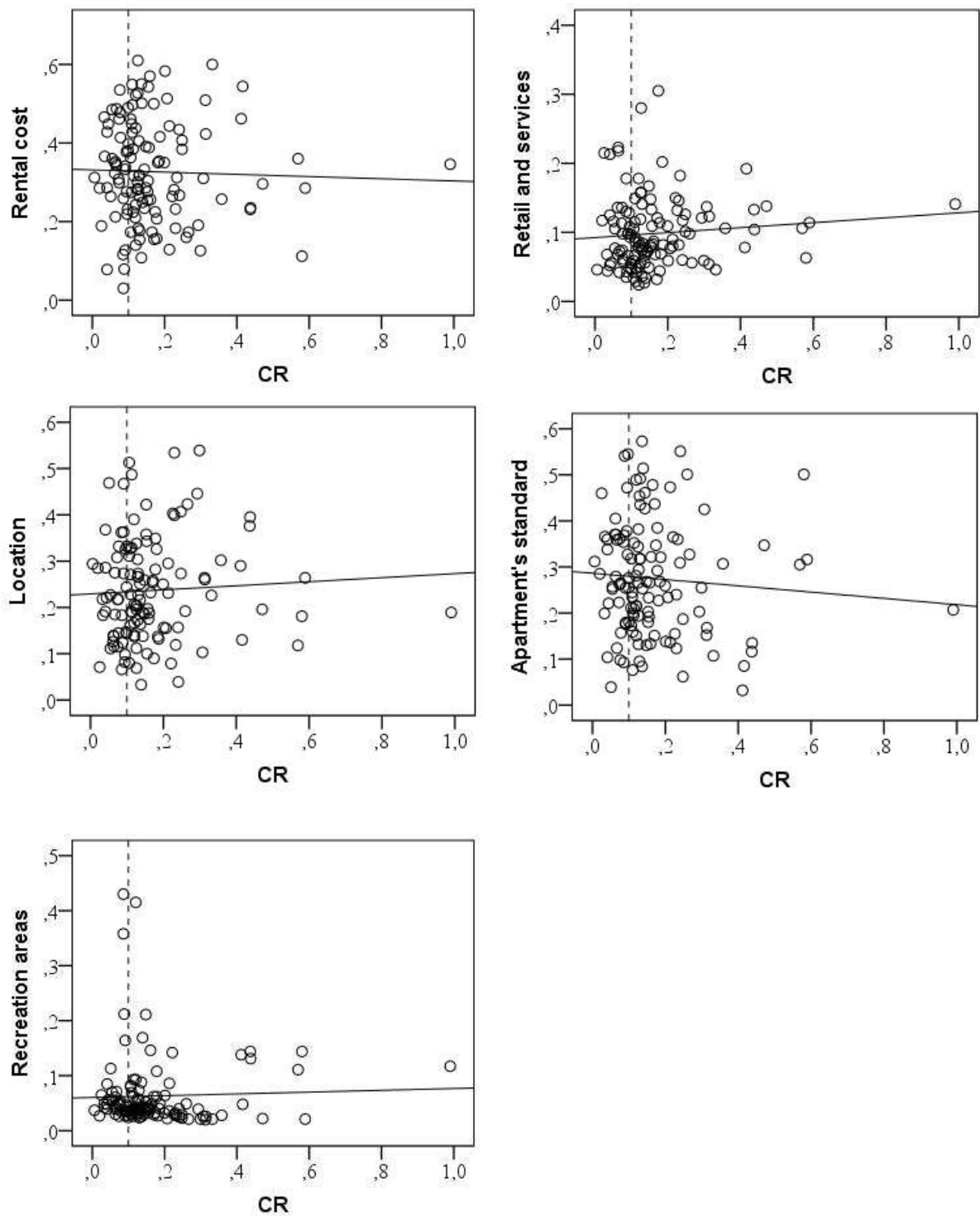
Figure 3. Consistency Ratio vs Criterion Weights
