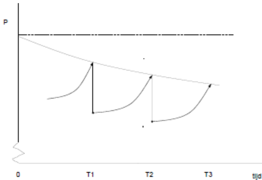
Figure 4.1 Optimal flooding probability should fall over time in line with economic growth and following a saw tooth-pattern (figure 2.4, p. 41 in Eijgenraam, 2005). Three lines are shown: 1) constant flooding probability, 2) flooding probability falling in time because economic growth leads to extra safety benefits and 3) optimal flooding probability which is falling over time and with a saw tooth-pattern: directly after the investment flood probability substantially drops, but after some time with economic growth this flood probability rises and then new investments in safety are needed.
