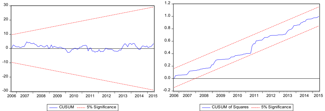
Figure 1: CUSUM and CUSUMQ of PSR model
