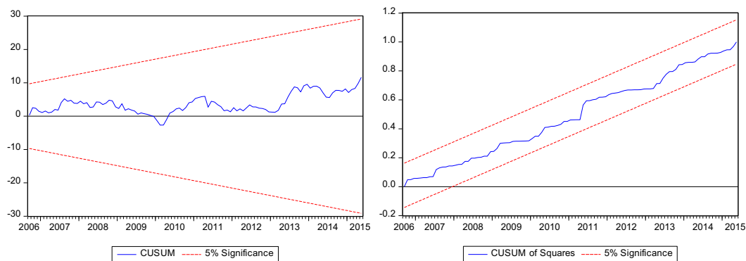
Figure 2: CUSUM and CUSUMQ of IR model
