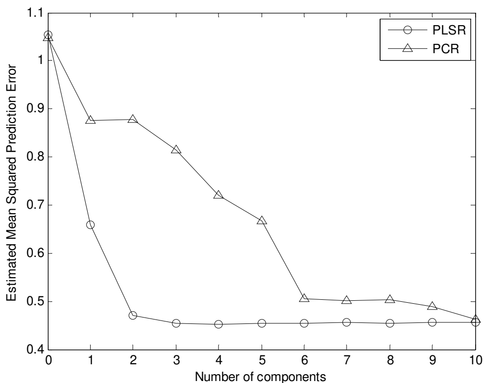
Figure 6.3: Estimated mean squared prediction error of PCR and PLSR depending on the number of latent components
