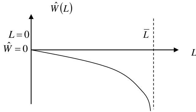
Figure 7: Zero welfare (no welfare) is a genuine maximum at no labor ( L=0 ), of the welfare function \hat{W}(L) .
