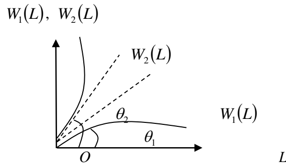
Figure 5: The behavior of the functions W_1(L) and W_2(L) for \theta_1 < \theta_2 .
