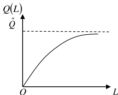
Figure 2: The function Q(L) represents the asymptotic curve of output \hat{Q} .
