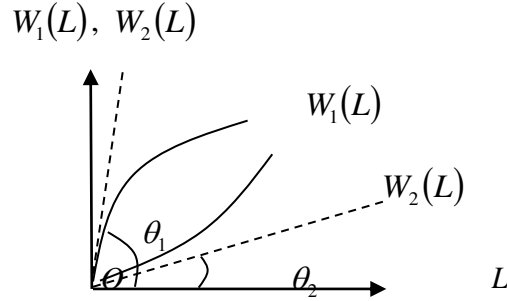
Figure 4: The behavior of the functions W_1(L) and W_2(L) for \theta_1 > \theta_2 .
