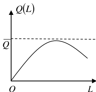
Figure 1: The function Q(L) represents the curve of maximization output \bar{Q} .
