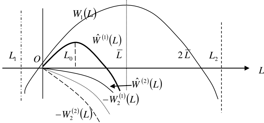
Figure 6: Nature of the functions W_1(L) , \hat{W}^{(1)}(L) , \hat{W}^{(2)}(L) , -W_2^{(1)}(L) and -W_2^{(2)}(L) are displayed.
