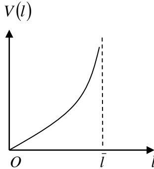
Figure 3: The function V(l) is asymptote at l = \bar{l} .
