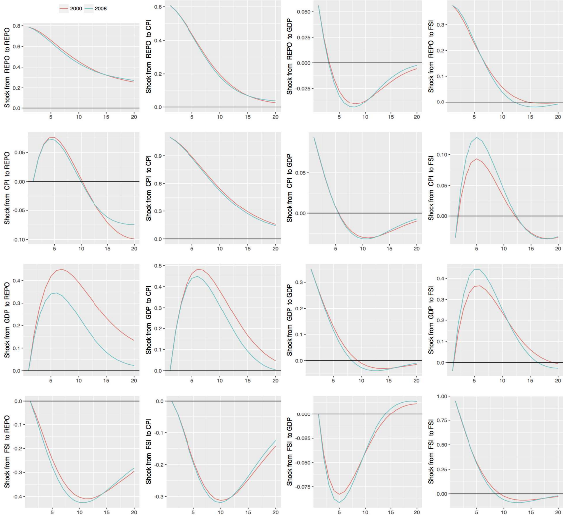
Figure 4: Comparison of impulse response functions
