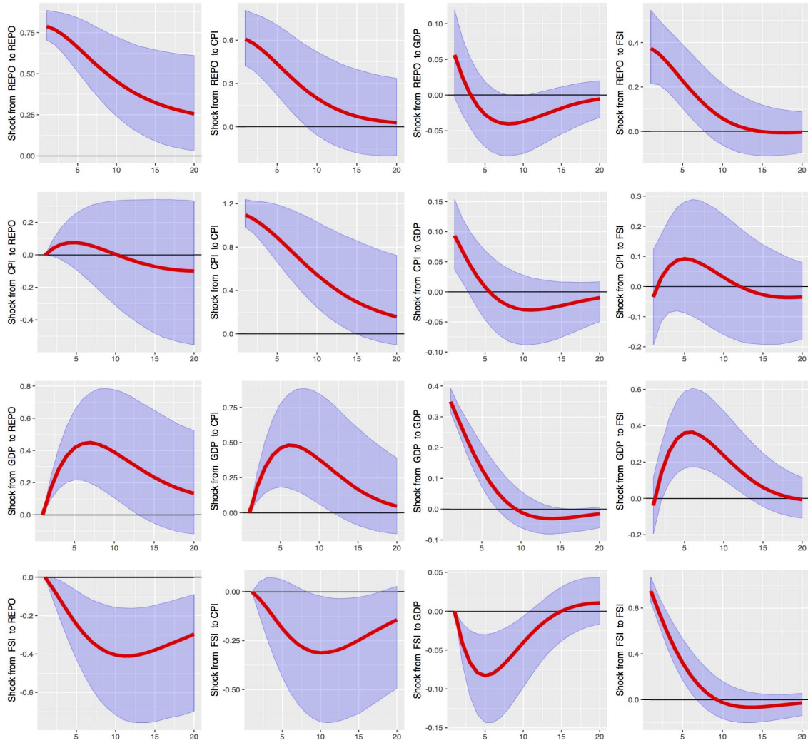
Figure 2: 2000-2007 Impulse response functions
