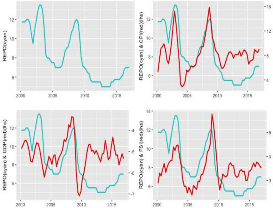
Figure 1: Plots of the variables
