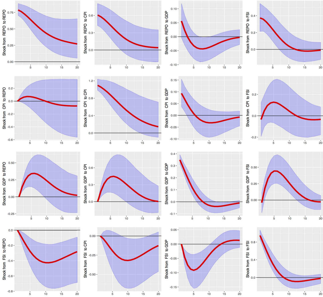
Figure 3: 2008-2016 Impulse response functions
