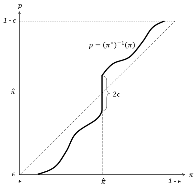
Figure 1: Prediction Market Equilibrium in the P - \pi Diagram.
