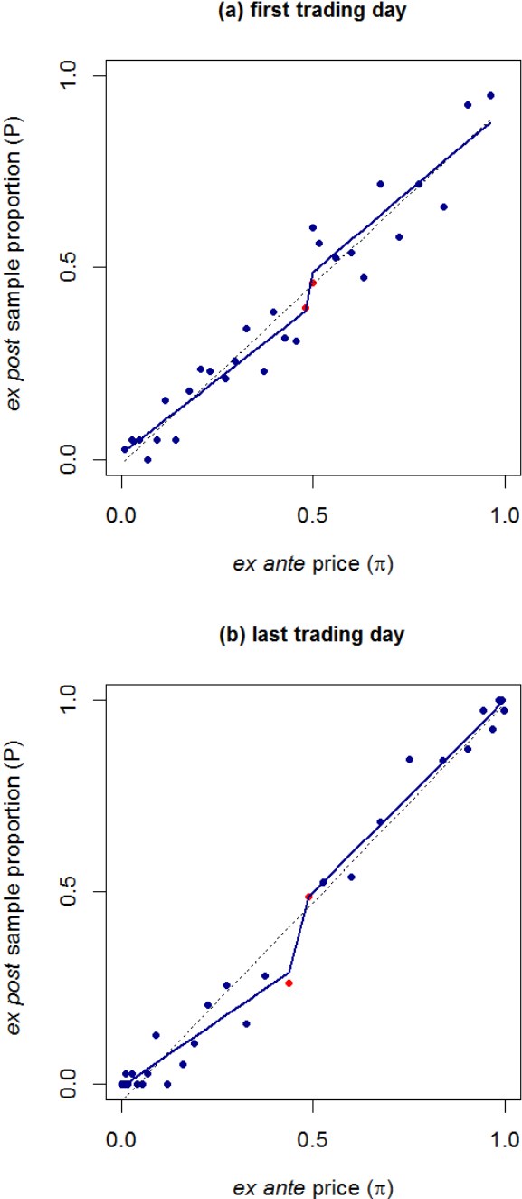
Figure 5: Prediction Market Data in the P - \pi Diagram: Entertainment (30 bins).
