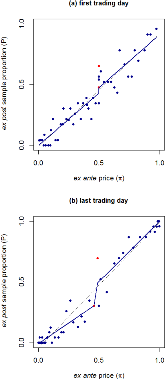
Figure 4: Prediction Market Data in the P - \pi Diagram: Entertainment (50 bins).
