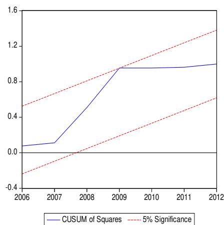
Fig. 2. Cusum of Squares
