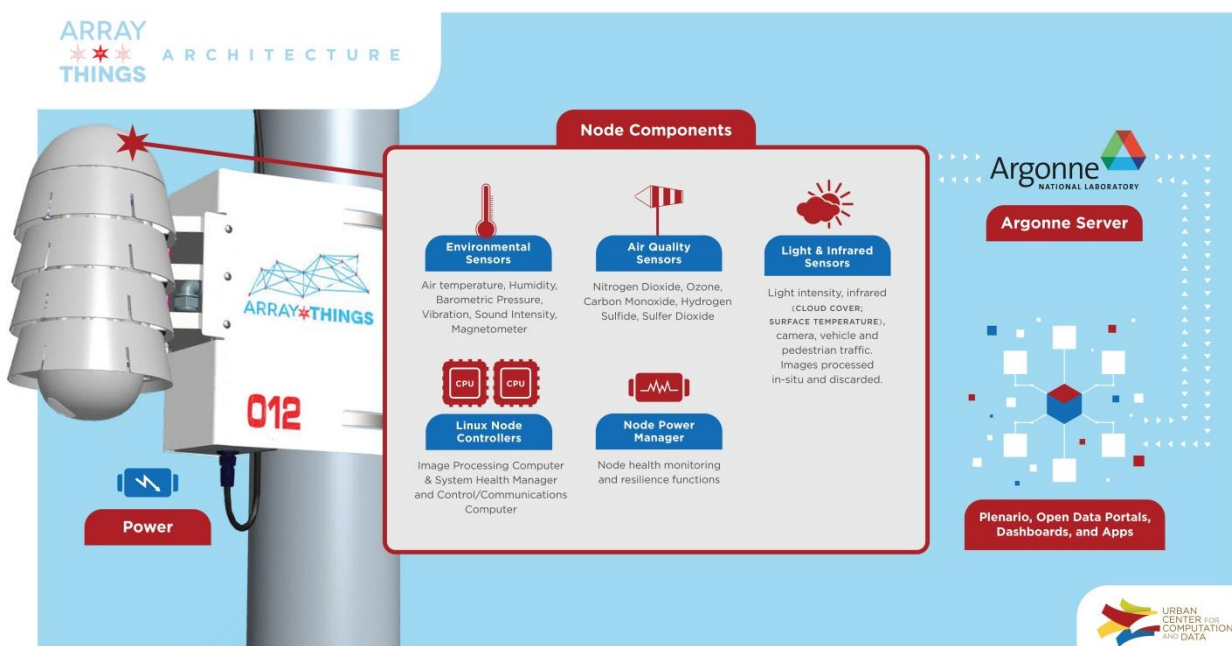
Fig. 2. Architecture of the Array of Things system [1]
