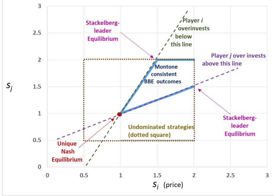
Figure 1: The Set of Monotone Consistent BBE Outcomes in Example 2 ( t = 1 , M = 3 )
