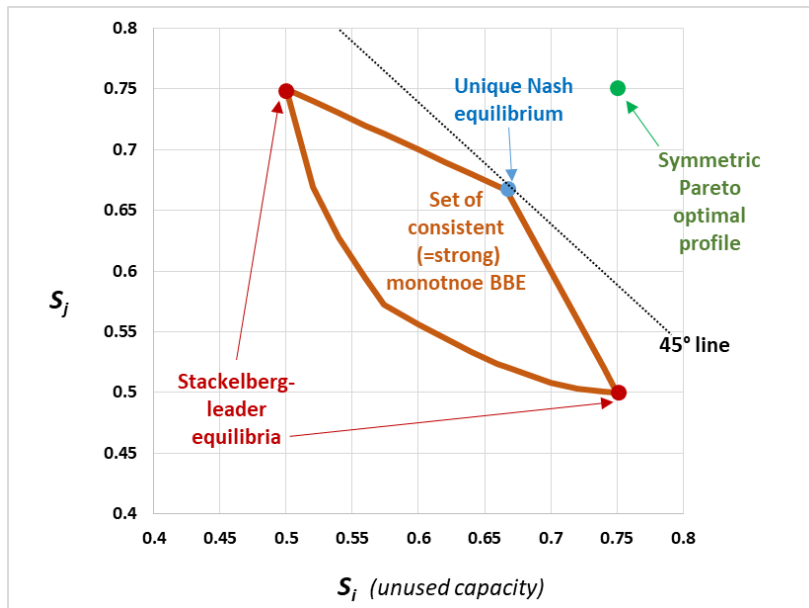
Figure 2: The Set of Monotone Consistent BBE Outcomes in a Cournot Competition
