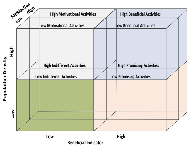
Figure 2: TiCoSa Model
