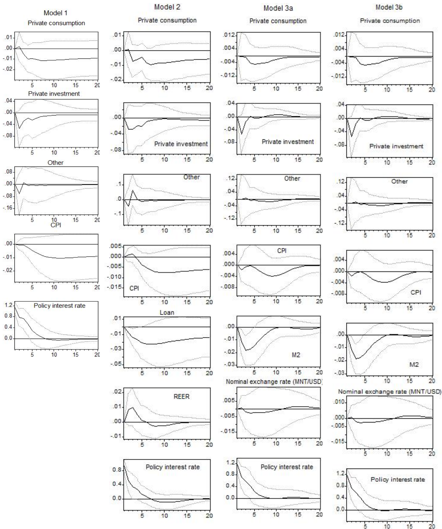
Figure 1: Impulse responses of tightening monetary policy shock (one standard deviation of the policy interest rate). Solid line is the impulse responses and dashed lines illustrate confidence intervals which are drawn using 10 th and 90 th percentile values of 1000 bootstrap simulations; All variables except policy interest rate are in log form (or %).
