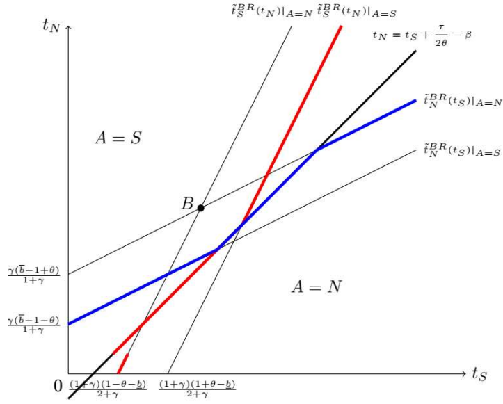
Fig. A15. Nash equilibrium for \tau < \tau_1 .
