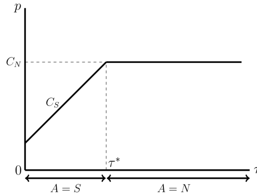
Fig. A1. Final good’s price under high unbundling costs.
