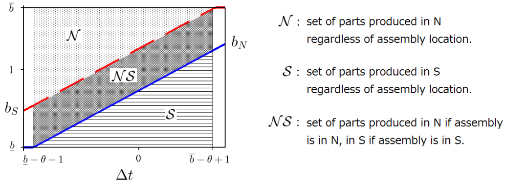
Fig. 2. Sourcing pattern under low unbundling costs.
