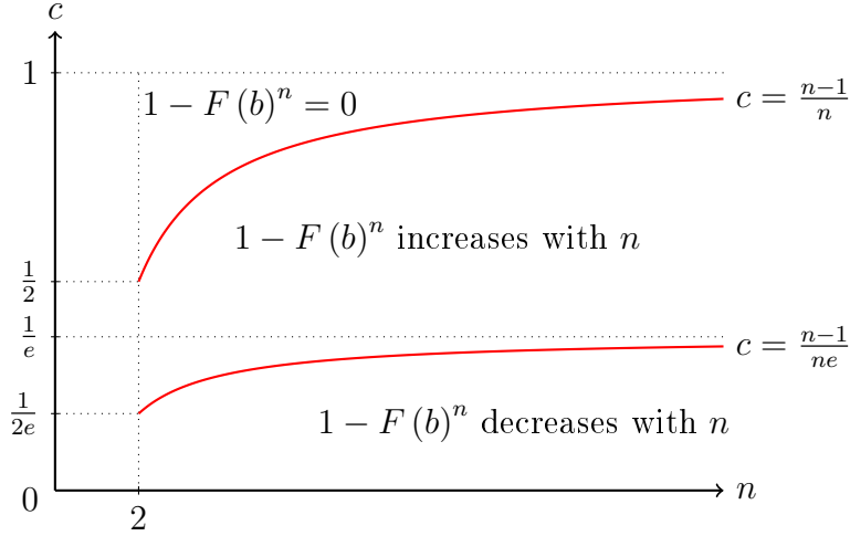
Figure 1: Effect of competition on F(b)^n .
